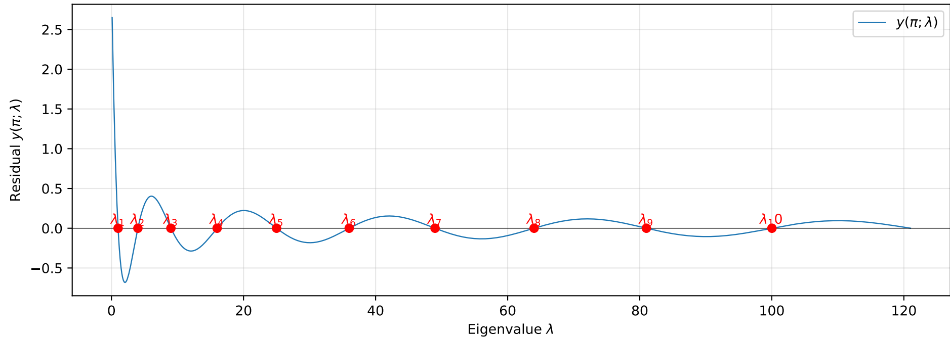
Residual sweep on uniform grid (n=100) for 10 eigenvalues
